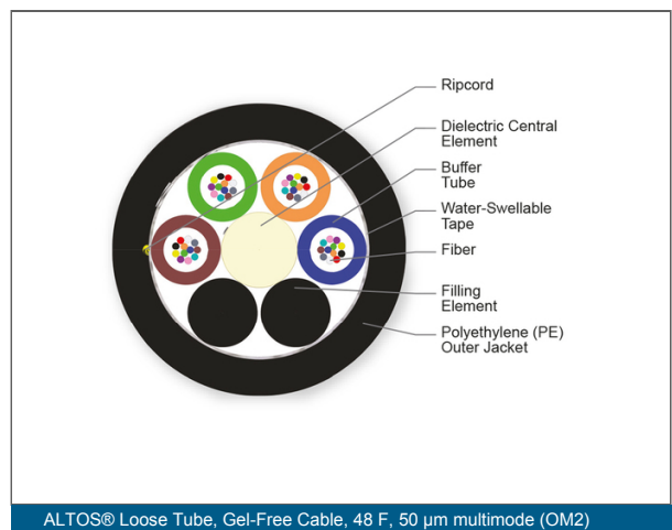
ALTOS® Loose Tube, Gel-Free Cable, 48 F, 50 µm multimode (OM2)
