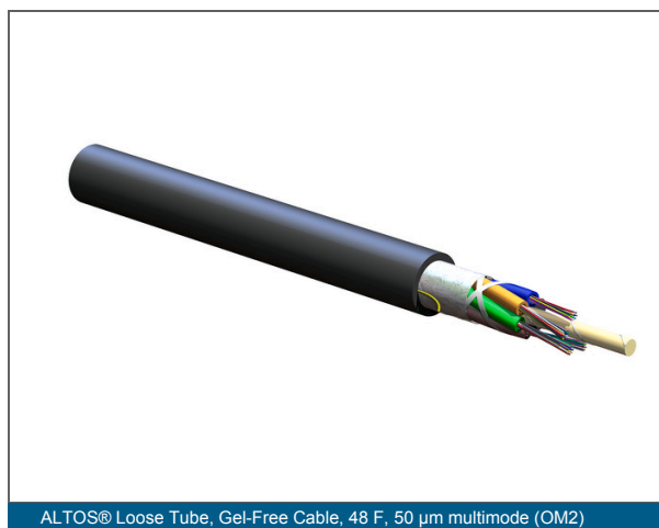
ALTOS® Loose Tube, Gel-Free Cable, 48 F, 50 µm multimode (OM2)
